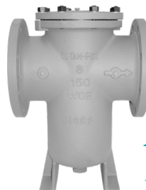
BS 85-CS BS 85-SS Class 150 Flanged Sizes: 2 ~ 12"
