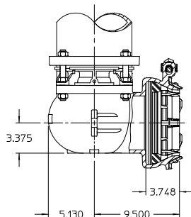
6 INCH ALPHA™ CONNECTION ALPHA™ is a licensed trademark of Romac Industries, Inc. (U.S. Patent 8,894,100)
