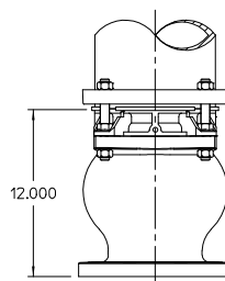
6 INCH FLANGED VERTICAL ENTRY CONNECTION
