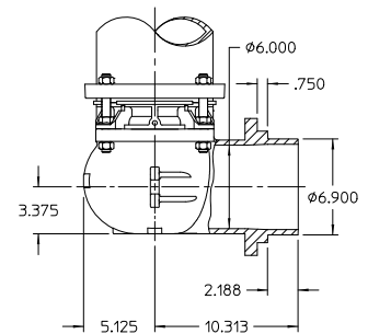
6 INCH PLAIN END W/INTEGRAL MJ GLAND CONNECTION
