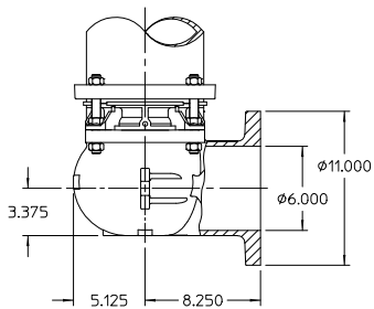
6 INCH CLASS 125 ANSI FLANGED CONNECTION
