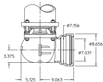
6 INCH TYTON® JOINT CONNECTION TYTON® is a registered trademark of United States Pipe and Foundry Co., LLC.
