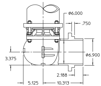
6 INCH PLAIN END W/INTEGRAL MJ GLAND CONNECTION
