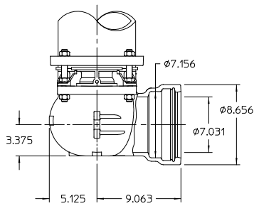
6 INCH TYTON® JOINT CONNECTION TYTON® is a registered trademark of United States Pipe and Foundry Co., LLC.
