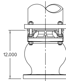
6 INCH FLANGED VERTICAL ENTRY CONNECTION
