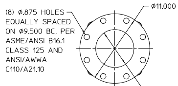
6 INCH FLANGED VERTICAL ENTRY CONNECTION
